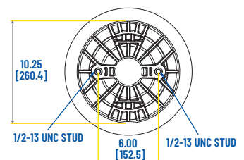
LOWER MOUNTING VIEW
