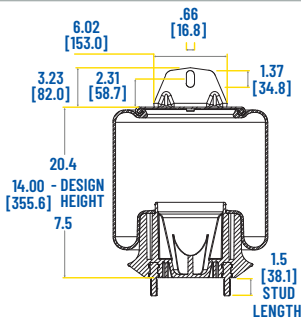
SIDE VIEW HEIGHT AND WIDTH
