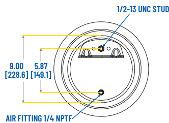
UPPER MOUNTING VIEW
