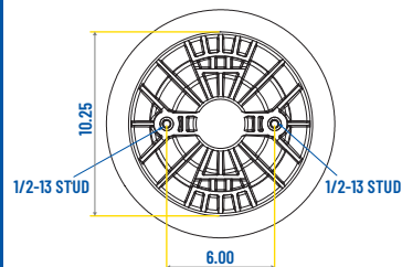
LOWER MOUNTING VIEW
