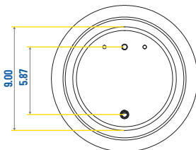
UPPER MOUNTING VIEW
