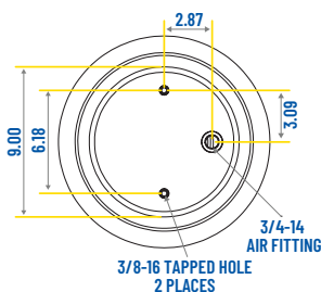
UPPER MOUNTING VIEW
