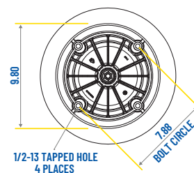
LOWER MOUNTING VIEW
