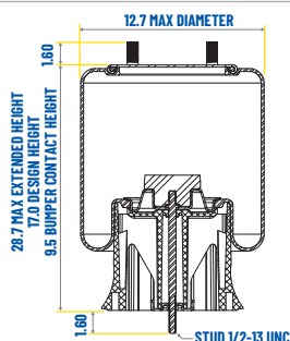
SIDE VIEW HEIGHT AND WIDTH
