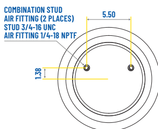
UPPER MOUNTING VIEW
