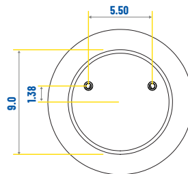
UPPER MOUNTING VIEW
