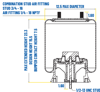
SIDE VIEW HEIGHT AND WIDTH
