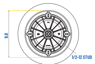
LOWER MOUNTING VIEW
