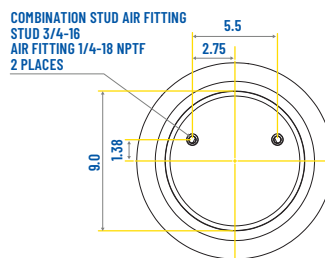
UPPER MOUNTING VIEW
