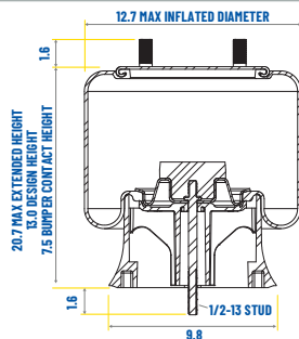
SIDE VIEW HEIGHT AND WIDTH
