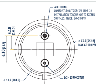
UPPER MOUNTING VIEW
