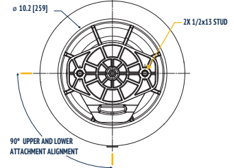
LOWER MOUNTING VIEW
