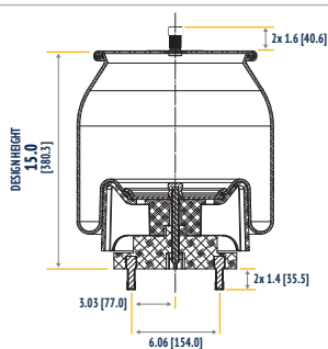
SIDE VIEW HEIGHT AND WIDTH
