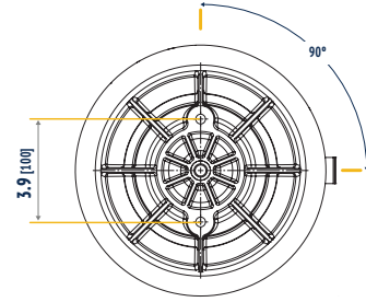
LOWER MOUNTING VIEW
