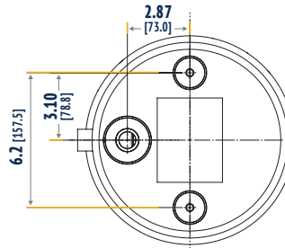
UPPER MOUNTING VIEW
