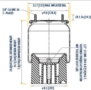
SIDE VIEW HEIGHT AND WIDTH
