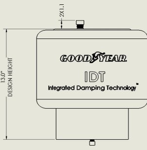
SIDE VIEW HEIGHT AND WIDTH
