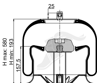
Cross Section
