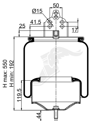
Cross Section
