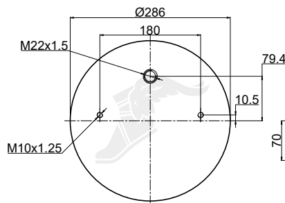
Upper Bead Plate
