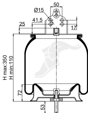
Cross Section
