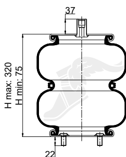
Cross Section
