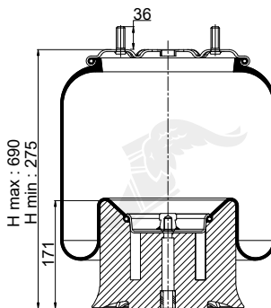
Cross Section
