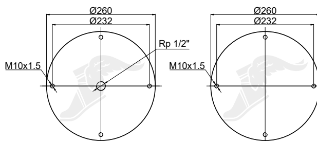
Upper Bead Plate
