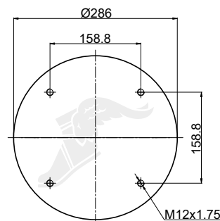
Lower Bead Plate
