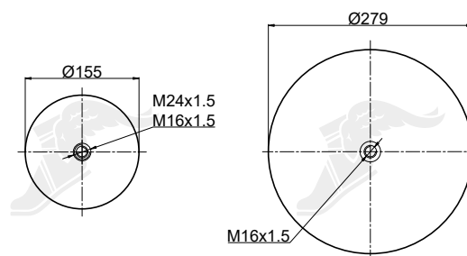
Upper Bead Plate
