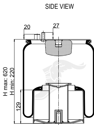
Cross Section
