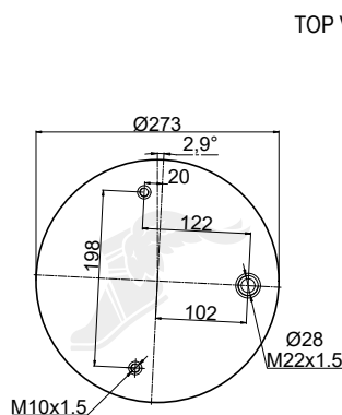
Upper Bead Plate
