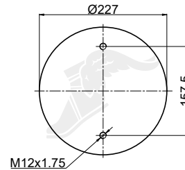
Lower Bead Plate
