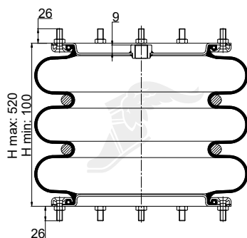
Cross Section
