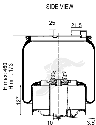
Cross Section
