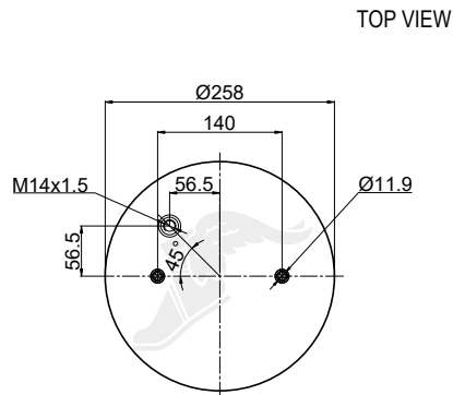
Upper Bead Plate
