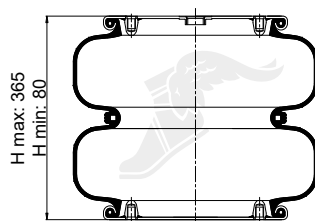
Cross Section
