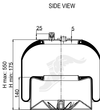
Cross Section
