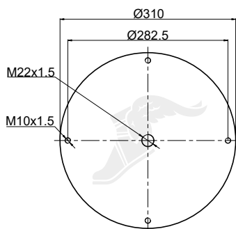
Upper Bead Plate
