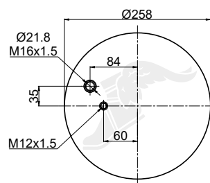
Upper Bead Plate
