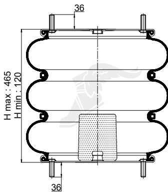
Cross Section
