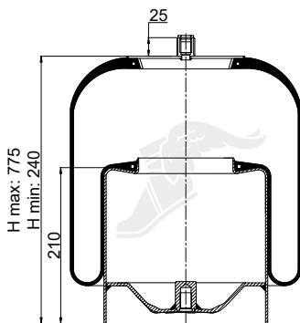
Cross Section
