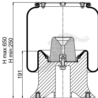
Cross Section
