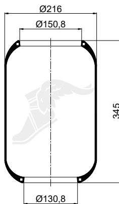
Cross Section
