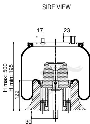
Cross Section
