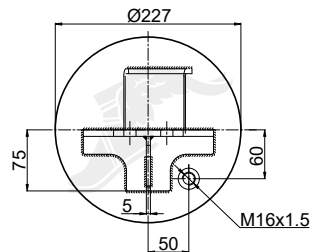
Upper Bead Plate
