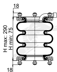
Cross Section
