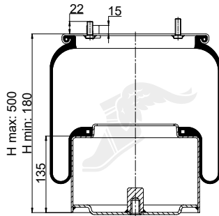
Cross Section
