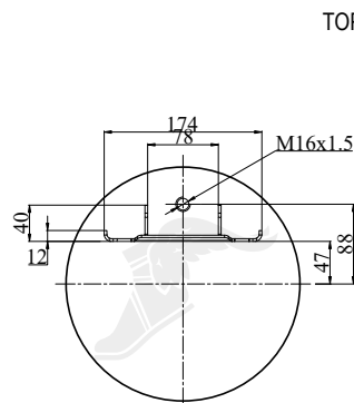
Upper Bead Plate
