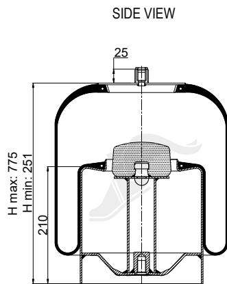
Cross Section
