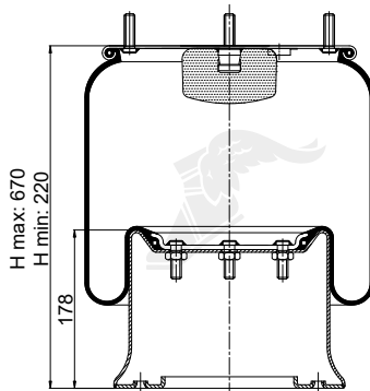
Cross Section
