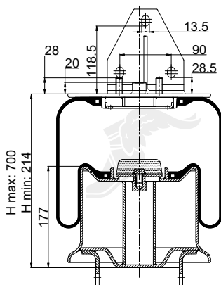
Cross Section
