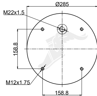
Upper Bead Plate
