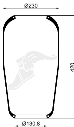
Cross Section
