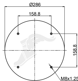
Lower Bead Plate
