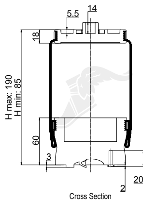
Cross Section
