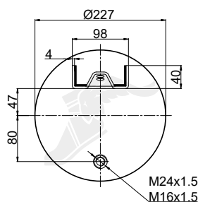
Upper Bead Plate
