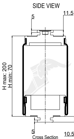
Cross Section
