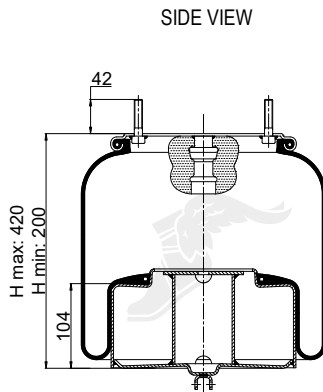
Cross Section
