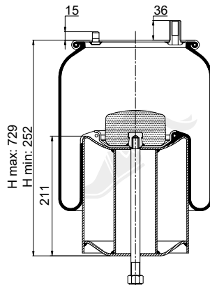
Cross Section
