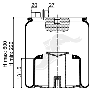
Cross Section
