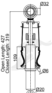
Cross Section
