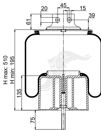
Cross Section
