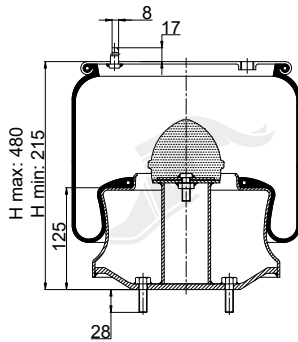
Cross Section
