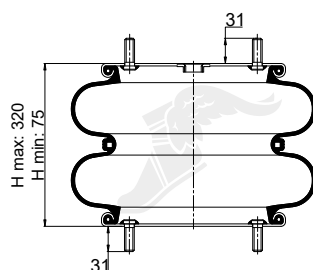
Cross Section
