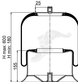
Cross Section
