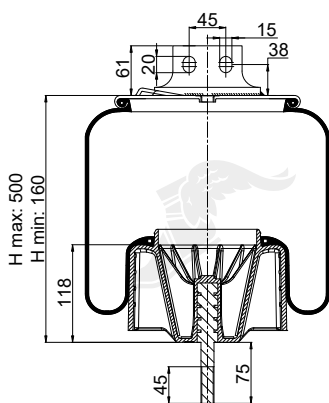
Cross Section
