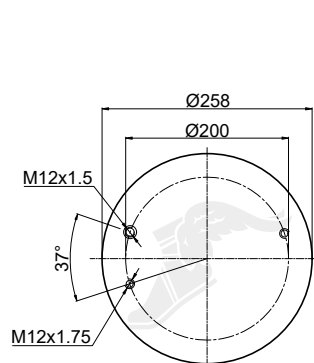
Upper Bead Plate
