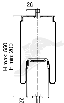
Cross Section
