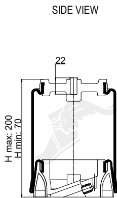
Cross Section
