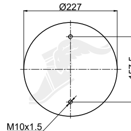
Lower Bead Plate
