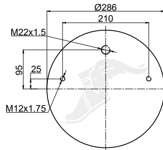
Upper Bead Plate
