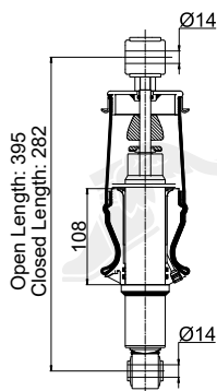
Cross Section
