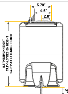
SIDE VIEW HEIGHT AND WIDTH
