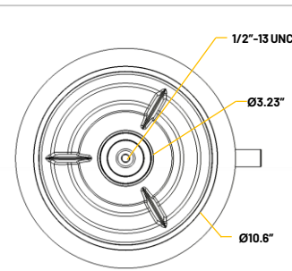
LOWER MOUNTING VIEW
