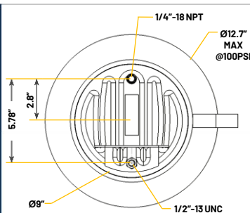
UPPER MOUNTING VIEW
